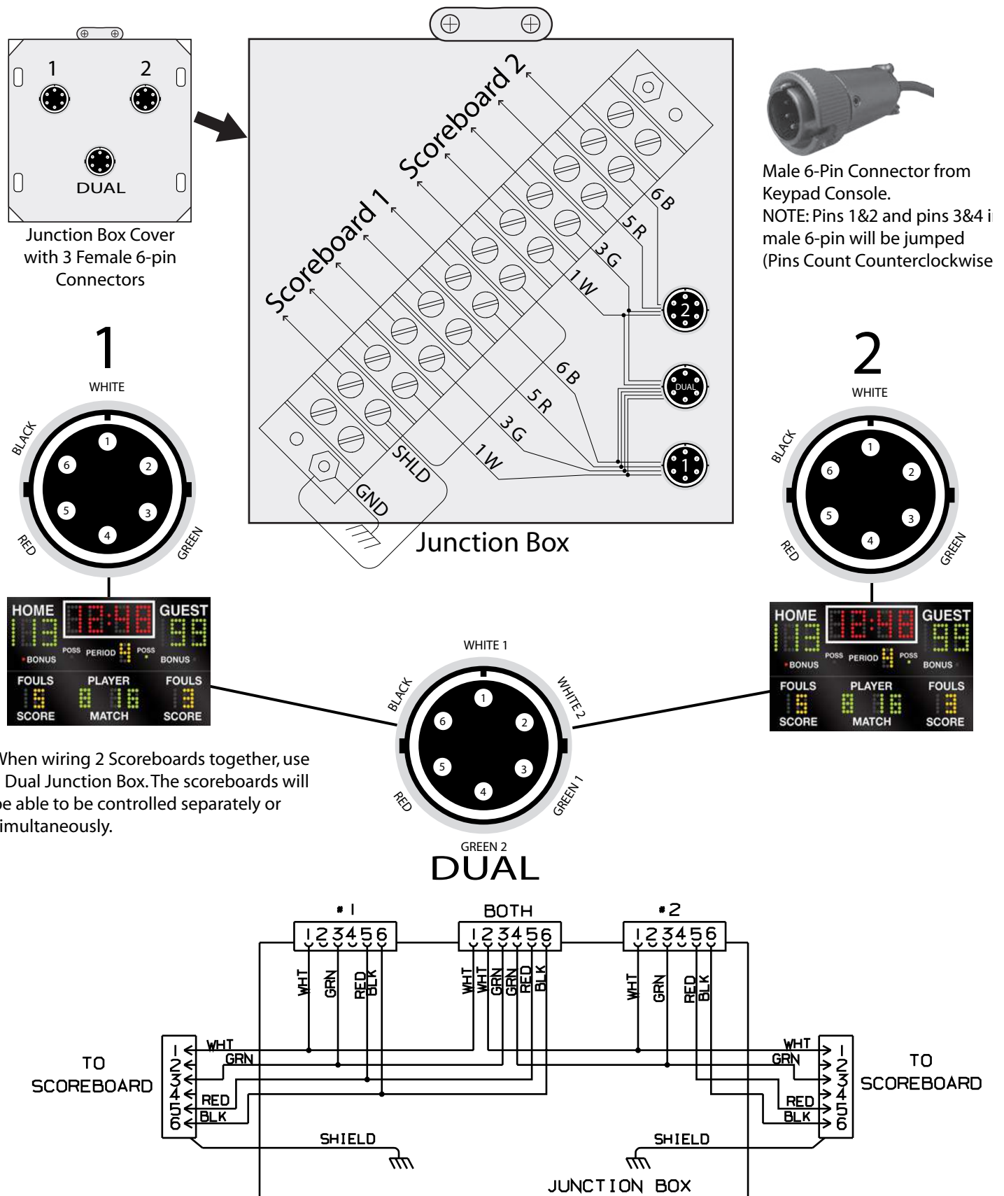
DUAL JUNCTION BOX WIRING
