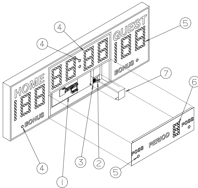
Figure 1 DISPLAY ASSEMBLY
