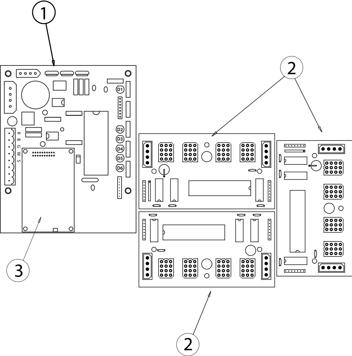
figure 2 CONTROLLER ASSEMBLY
